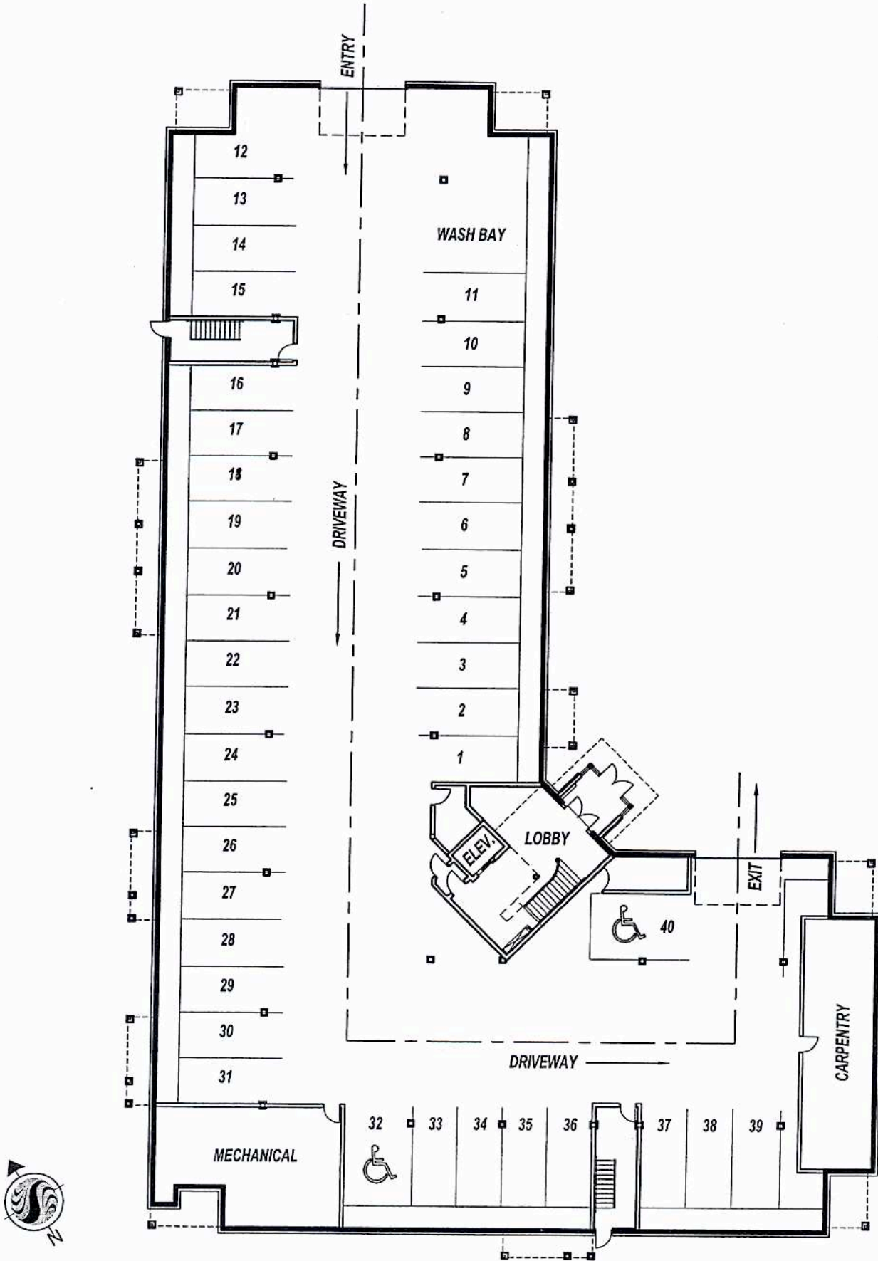
MAIN FLOOR PLAN/PARCADE
